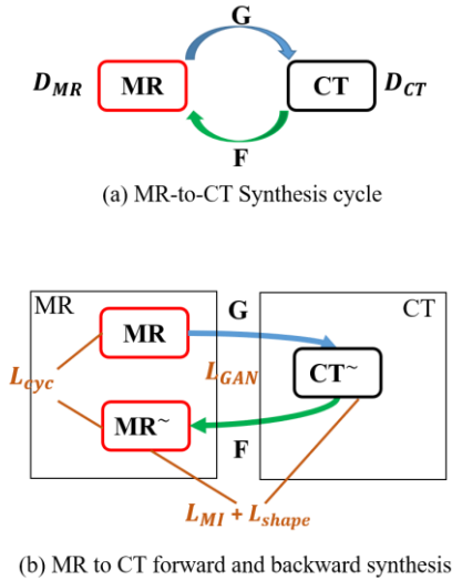
Fig. 1. Schematic illustration of: (a) the conventional Cycle-GAN algorithm, and (b) the forward and backward synthesis step of the proposed method with MI and SC as the direct structural similarity constraint.
